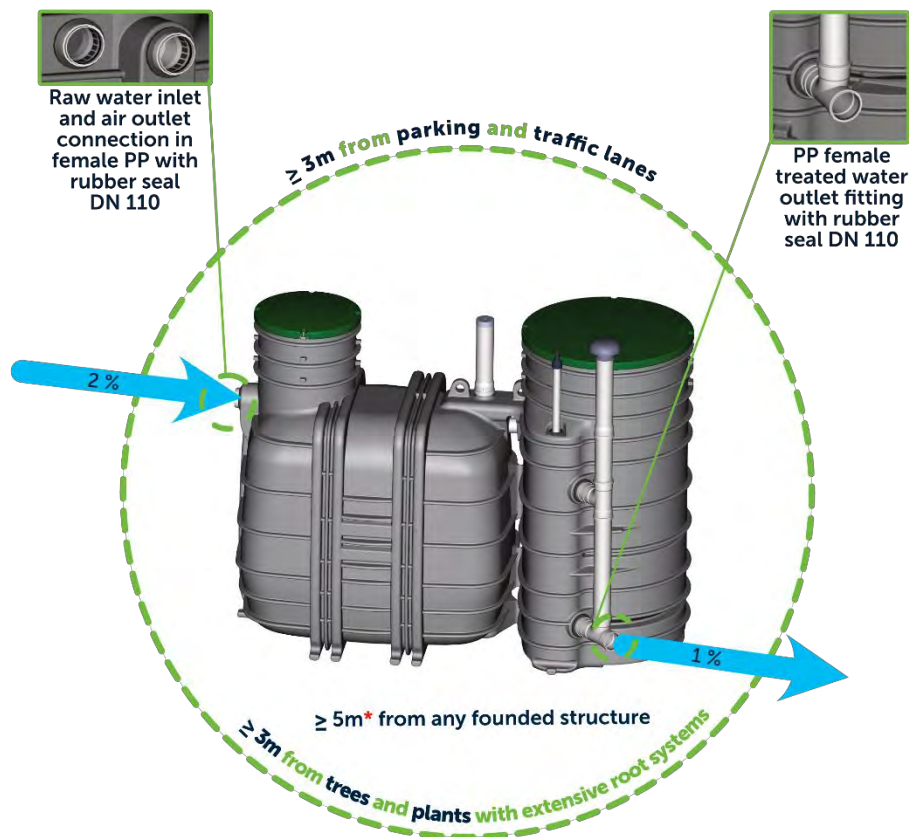
Installation recommendations
