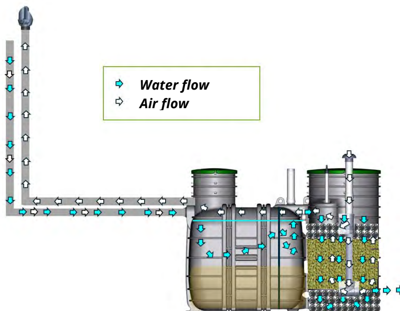
Diagram of the water circulation and ventilation
